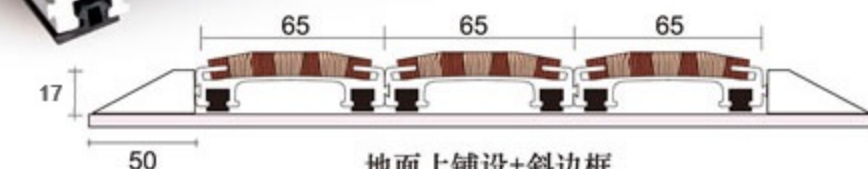
地面上铺设+斜边框 Installation aground + Beveled edges
